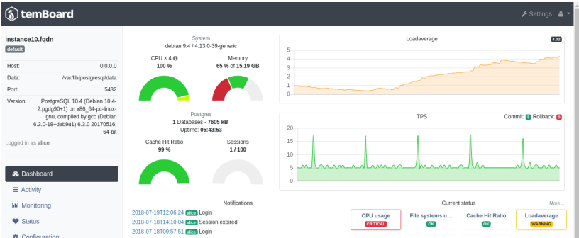
Figure 1: temBoard UI
